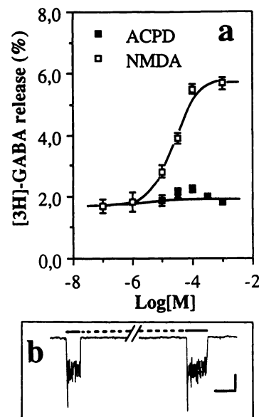
Fig. 4. ACPD did not activate NMDA receptors in cultured striatal neurons. a , The release of [^3\text{H}]\text{GABA} from striatal neurons was determined as described in Experimental Procedures, in the absence of \text{Mg}^{2+} . The percentage of radioactivity released from the cells was measured after a 4-min stimulation with increasing concentrations of NMDA or ACPD. Results are means \pm standard errors of triplicate determinations. Similar results were obtained twice. b , The whole-cell recording (digitized at 17\text{ Hz} ) was obtained from one neuron, in the absence of \text{Mg}^{2+} and in the presence of 1\text{ }\mu\text{M} glycine, at a holding potential of -60\text{ mV} . The two NMDA ( 100\text{ }\mu\text{M} ) applications (—) were separated by a 5-min application of ACPD ( 100\text{ }\mu\text{M} ) (---). Calibration bars, 50\text{ pA} and 10\text{ sec} . Similar results were obtained from five other cells.
