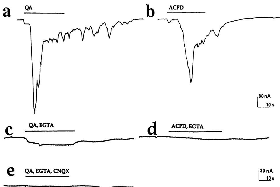
Fig. 2. Stimulation by ACPD of Q_p but not of QA/KA receptors in Xenopus oocytes previously injected with rat brain RNA. Oocytes were voltage clamped at -80 mV. Agonists were applied directly in the bath using a 20\text{-}\mu\text{l} pipette, with the perfusion being stopped. The time of stimulation is indicated by the bars above the current traces. The concentrations of pharmacological agents were 100\text{ }\mu\text{M} and 1\text{ mM} for QA and ACPD, respectively. When indicated, 50\text{ nl} of EGTA ( 20\text{ mM} , pH 7) were injected into the oocyte with a Drummond micropipette, leading to an intracellular concentration in the range of 0.5\text{ mM} . All experiments were performed on the same oocyte and repeated three times.
