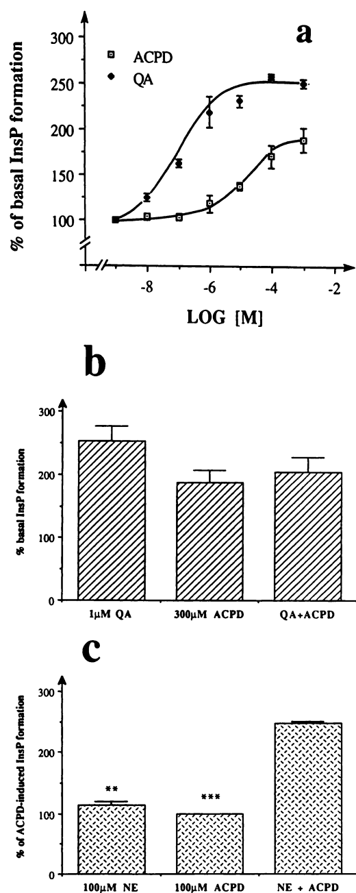
Fig. 1. Stimulation by ACPD and QA of InsP accumulation in cultured striatal neurons. a , Dose-response curve for ACPD stimulation of InsP accumulation. Values represent means \pm standard errors of three independent experiments, in which each data point was obtained in duplicate. Basal InsP accumulation was 930 \pm 39 dpm. b , Nonadditivity of ACPD and QA effects on InsP accumulation. Basal InsP accumulation was 1370 \pm 51 dpm. c , Additivity of ACPD and NE effects on ACPD-induced InsP accumulation. Basal InsP accumulation was 1134 \pm 43 dpm. Values of NE, ACPD, and NE plus ACPD were significantly different (**, p < 0.03 ; ***, p < 0.001 ), as determined with Student's t test.
